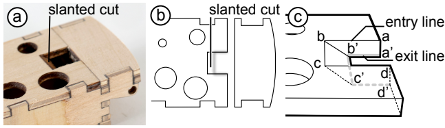
Figure 6: (a) When encoding this ocarina model for 5DOF laser cutting, (b) existing SVG-based designs (black) are combined with features (black/gray) that require slanted cuts. (c) Each segment in an SVG5DOF file defines a tool path as the linear interpolation between entry line and exit line.
