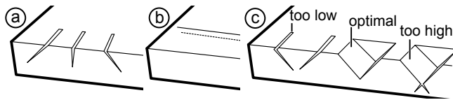
Figure 5: Calibration patterns for (a) tilt center, (b) table center, and (c) cutting depth
