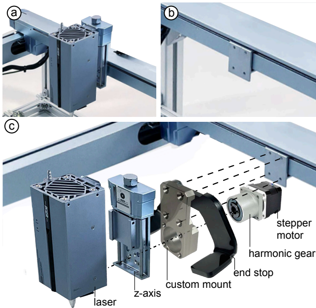
Figure 3: We added head tilt to an off-the-shelf laser cutter [34] by (a) removing the laser head and z-axis from the gantry, then (b) using the exposed mount (c) to insert a stepper motor and a gearbox, held together by a custom mount.
