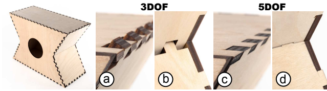
Figure 18: Angled box joints cut with 3DOF have gaps in (a) acute and (b) concave edges. 5DOF laser cutting (c, d) creates flush, angled box joints by cutting at the same angle the joint will meet, here shown on a slap-top cajon.
