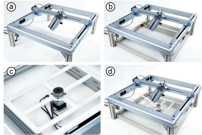
Figure 4: (a) We added yaw by (b) extending the casing with a mount, (c) mounting a stepper motor and zero-backlash gearbox, and (d) adding the round table.
