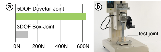
Figure 17: (a) Test setup. (b) Dovetail joints withstood 5.8x higher loads than “hand-tight” box joints.
