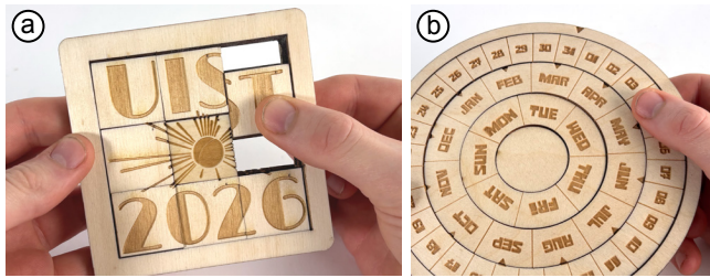
Figure 25: Cut-in-place sliding mechanisms allow creating parts with (a) multiple moving pieces (here, a sliding puzzle) and (b) rotary sliding mechanisms (here, a circular calendar).
