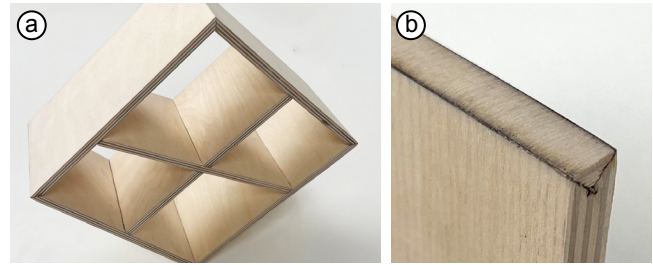
Figure 22: (a) Front and back of plate-based models continue to show the plywood's end grain. (b) 5DOF allows covering these up using a wedge-shaped “veneer”.
