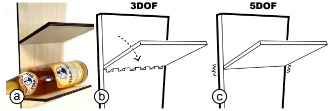
Figure 16: The fact that 5DOF allows cutting these T-joints at the correct angle allows them to take a load.
