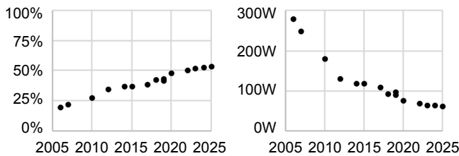
Figure 2: (a) Laser diode efficiency is continuing to grow, causing (b) waste heat (here for 70W output) and thus heatsinks to shrink exponentially (data aggregated from [41] and [50]).
