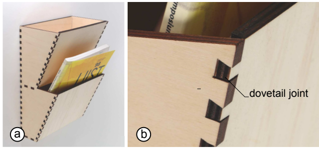
Figure 13: (a) Magazine rack created using our 5DOF prototype. (b) Dovetail joints prevent the front plate from falling out.
