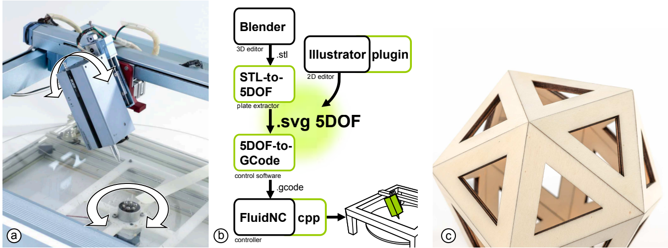
Figure 1: Can diode-based laser sources bring laser cutters capable of tilting their heads to makers, and if so, how to enable this? (a) To explore this question, we created a hardware prototype of a desktop 5DOF laser cutter from maker-available components. (b) We then created a toolchain for controlling the device exclusively by extending programs and file formats used by makers today. We extended the SVG file format to 5DOF and created four extensions and converters around it, here highlighted in green. (c) We then applied the prototype and the toolchain to maker-friendly materials, suggesting that future makers might use 5DOF machines to fabricate hidden joints (as well as load-bearing joints and cut-in-place mechanisms).
