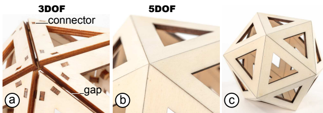
Figure 20: (a) This 3DOF model of an icosahedron desk lamp is held together by an internal support structure. (b) The 5DOF version based on miter joints requires no internal structure.
