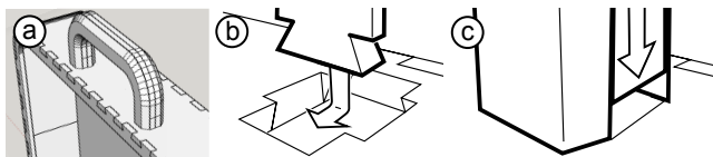
Figure 15: (a) This handle uses dovetail T-joints to withstand tension, which are inserted by (b) pushing the plate through a slot, then (c) sliding the plate into place to lock the joint.
